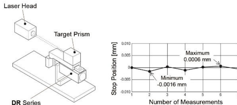
Fig. 6: The repeat positioning accuracy determined with a laser measurement is \pm 0.0011 mm, specified as \pm 0.003 mm at constant temperature and load.
