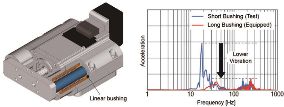
Fig. 3: Lower spindle vibrations by using longer guide bushes. Measurement in vertical direction of movement with 100 mm/s, 30 mm stroke and 2 kg load.
