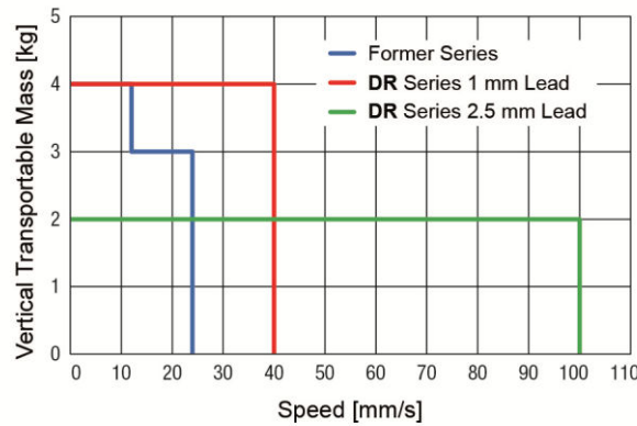
Fig. 5: The DR Series achieves speeds of up to 100 mm/s compared to the previous series.
