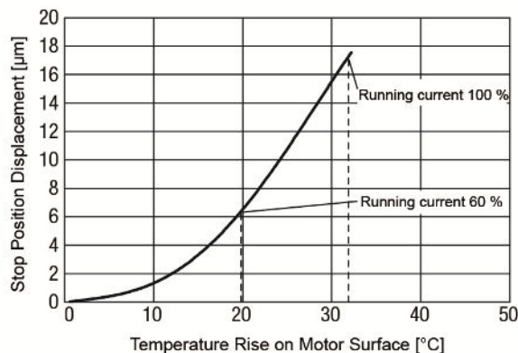
Fig. 9.: Improved stopping accuracy by reducing the operating current.
