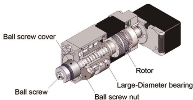
Fig. 2: Compact size through integration of hollow rotor and ball screw.
