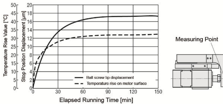
Fig. 7: The motor temperature increases with longer operating times, but this has only a minimal effect on the positioning accuracy of the DR Series with less than 18 micrometres.
